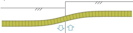
Fig.1: Numerical simulation of a buried pipeline crossing a fault
