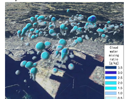
Simulated cumulous clouds over Kobe city
