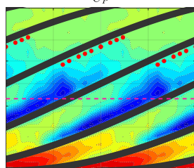
Pressure distribution around spiral protuberances
