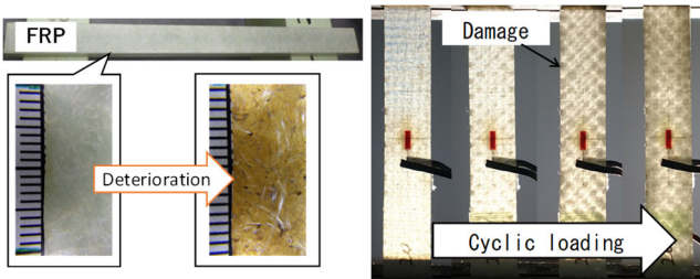
Evaluate aging and fatigue damage of fiber reinforced plastic (FRP) and reveal its effect on mechanical behavior
