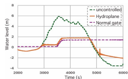
Tsunami Reduction Effect of the Hydroplane Tsunami Barrier
