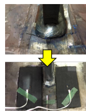
Evaluation of remaining fatigue life after CFRP bonded repair
