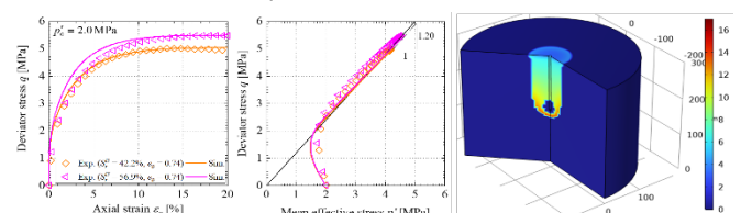
Left : Elasto-plastic constitutive equation for CO 2 hydrate soils
