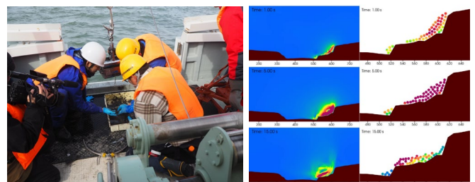
A scene from a submarine geotechnical survey (left) and a numerical simulation of a submarine landslide (right)
