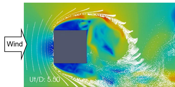
Air flow and particles around a rectangular prism
