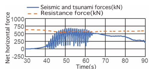
Time History of Net Horizontal Force on a Breakwater
