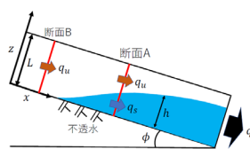
Modeling slope runoff processes
