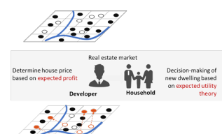
Flood exposure population simulation in Kyoto
