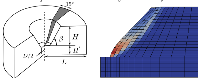
Fig. 2: Stability analysis of excavation
