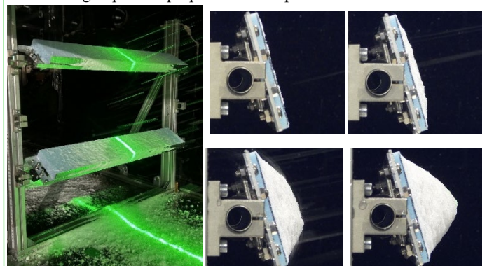
Snow accretion experiment on test plates (left) and temporal changes in the shape of snow accretion (right)
