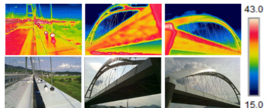
NDT technique for checking health condition of infrastructures by infrared camera
