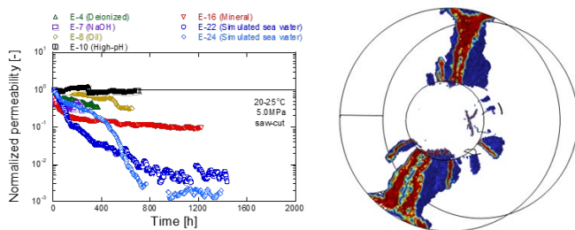
Continuous permeability tests and crack propagation analysis of hydraulic fracturing experiments
