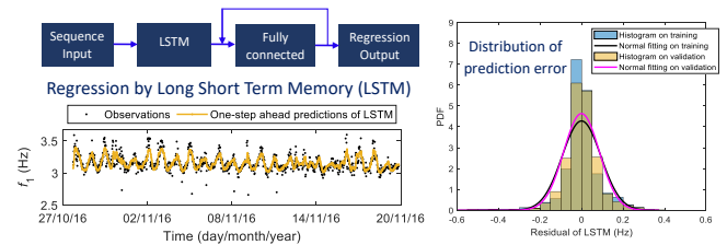
Fig. 3: Predicted frequency of a bridge under changing environment and error distribution of the prediction.
