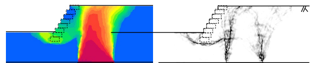
Fig. 5 : Laboratory investigation of tunnel-masonry interaction.
