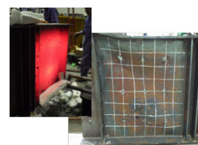
Heated steel girder after shear test
