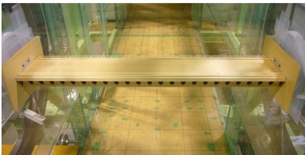
Bridge girder model with side openings for wind tunnel tests
