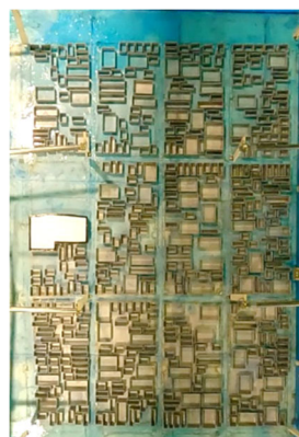
Simulation results on the inundation depth (above) and experimental results on urban flood inundation (right).
