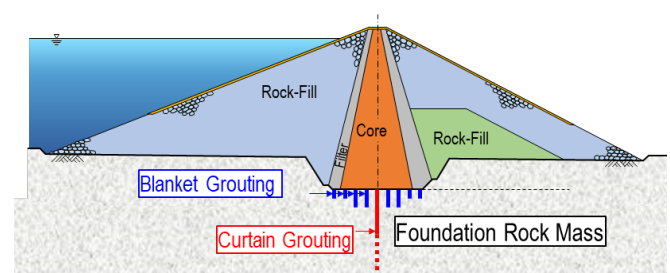
Concept of grouting in dam foundation
