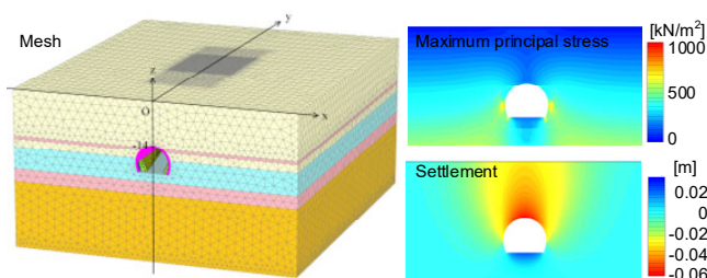
Excavation analysis of shallow overburden tunnel
