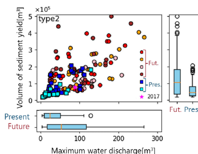
Fig. 2: Projection results of maximum water discharge and volume of sediment yields under rainfall events in present and future climate.
