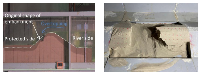
Experiments on the river dyke breach (left: one-dimensional flume in the cross-sectional direction, right: two-dimensional flood basin with river flow)
