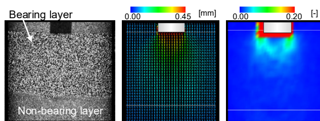
(a) CT image (b) Vertical disp. (c) Shear strain Bearing capacity of thin-layer supported pile using X-ray CT
