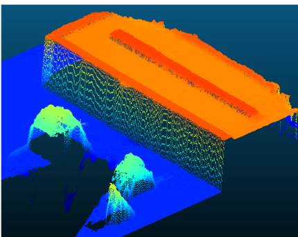
Reconstructed 3D map of the construction site in the above simulator. The achieved accuracy of objects is less than 10 cm.
