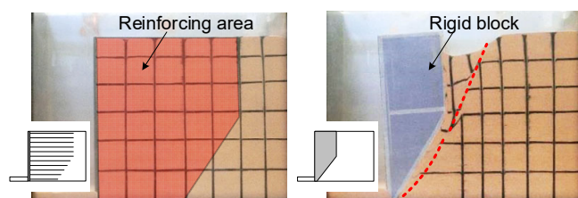
Seismic performance of reinforced earth wall (centrifugal model test)
