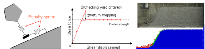
Simulation of seismic behaviors of rock slope using DDA
