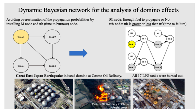
Figure 2. Dynamic Bayesian network for the analysis of domino effects at a storage tank farm following earthquakes.
